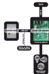
Phone Line Verifier (PLV)
